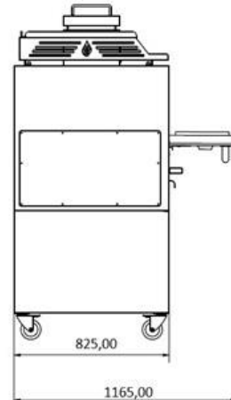
Dimensions with Open Door
