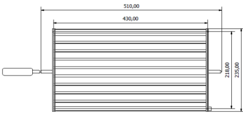
Basket Dimensions
