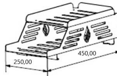
Gastronorm rack
