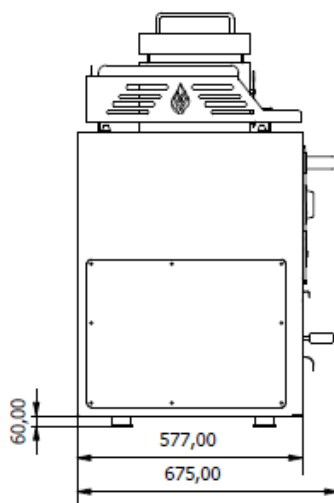
Roasting area
