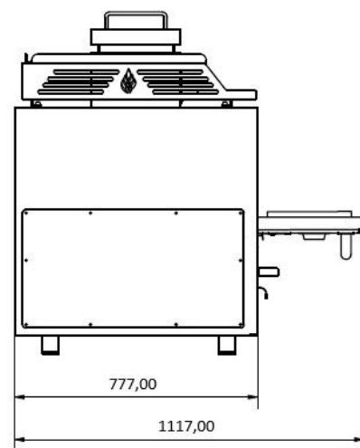
Gastronorm rack
