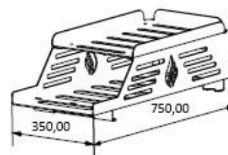
Gastronorm rack
