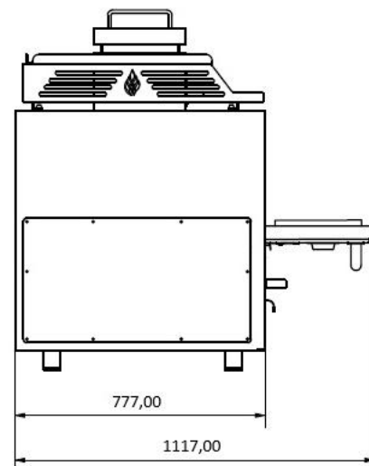
Gastronorm rack
