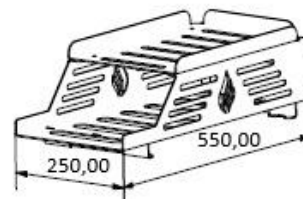
Gastronorm rack
